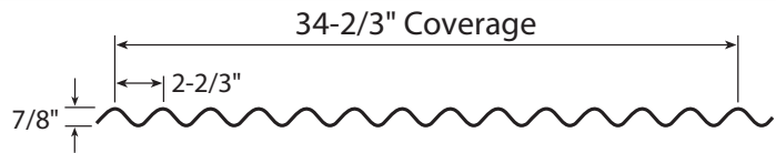
Wall Panel
