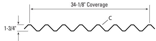
T12 Wall
