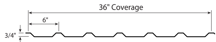
U-Panel
